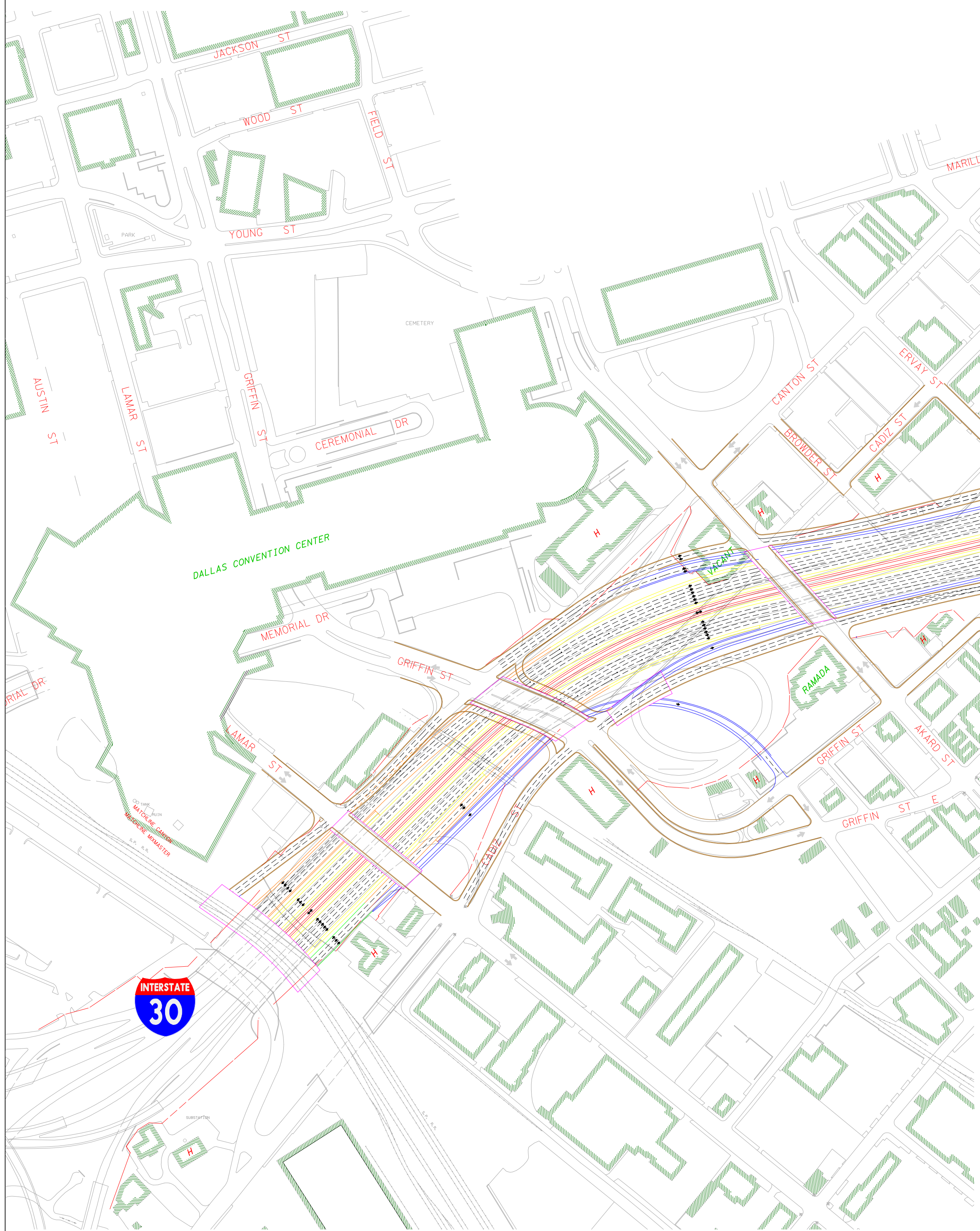
WESTBOUND I-30 BRAIDED RAMP ALTERNATIVE
